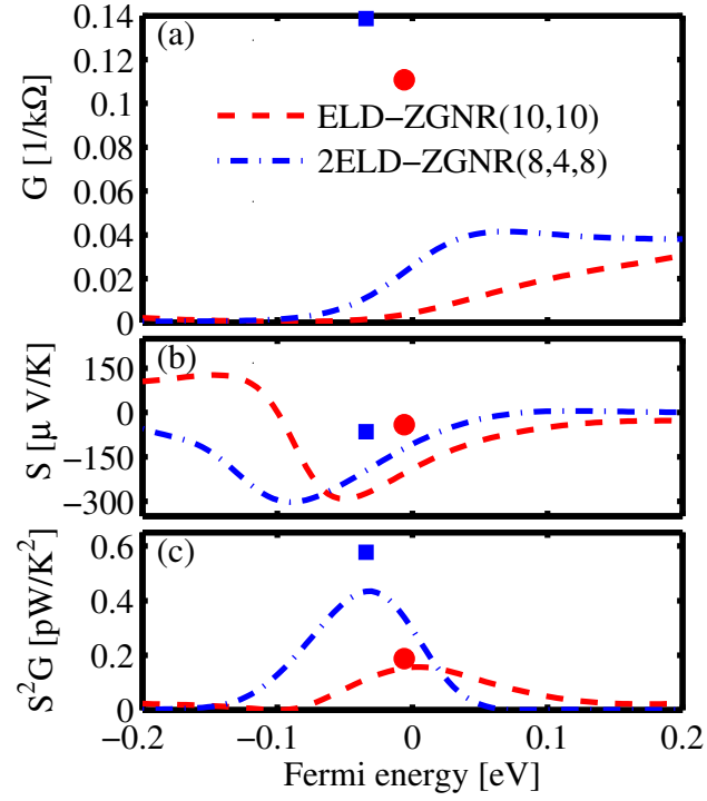
FIG. 10: (a) Electrical conductance, (b) Seebeck coefficient, and (c) thermoelectric power factor of ELD-ZGNR(10,10) and 2ELD-ZGNR(8,4,8) with rough edges and positively charged substrate impurities. The channel length is 2 \mu m . The dots indicate the Fermi energy values at which the peak of the power factor G occurs for the pristine ELD and 2ELD channels of Fig. 9 for comparison purposes.
