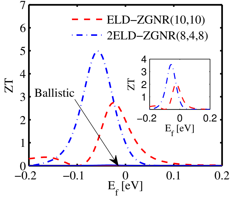
FIG. 11: The thermoelectric figure of merit ZT for the ELD-ZGNR(10,10) (dashed-red line) and 2ELD-ZGNR(8,4,8) (dash-dot-blue line) channels of length L = 2 \mu m . The lattice thermal conductance is extracted from the calculated mean free path. Inset: The same figure of merit ZT but with the lattice thermal conductance extracted by integrating the simulated phonon transmission.
