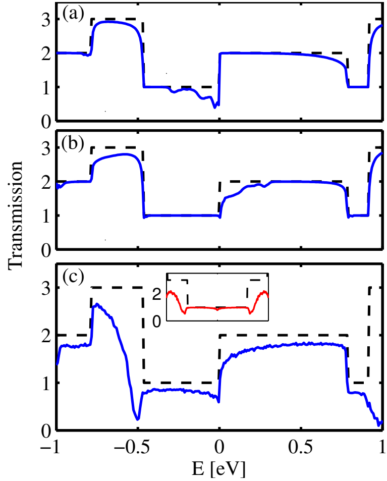
FIG. 4: The effect of (a) positive substrate impurity, (b) negative substrate impurity, and (c) roughness on the transmission of ELD-ZGNR(10,10) with length of 125 nm. Inset of (c): The transmission of ZGNR(20) in the presence of roughness.
