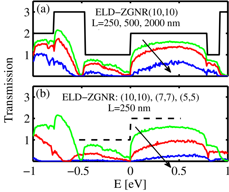
FIG. 5: The influence of roughness and positive impurities on the ELD-ZGNR channel. (a) Electronic transmission of ELD-ZGNR(10,10). Rough edges are assumed and the length L is varied. The arrow indicates increasing values of length L . (b) Electronic transmission of ELD-ZGNRs with different widths. The length is assumed to be constant at 250 nm and the arrow indicates the direction of decreasing the ribbon's width. Black-solid and black-dashed lines in (a) and (b): The transmission of the pristine ELD-ZGNR.
