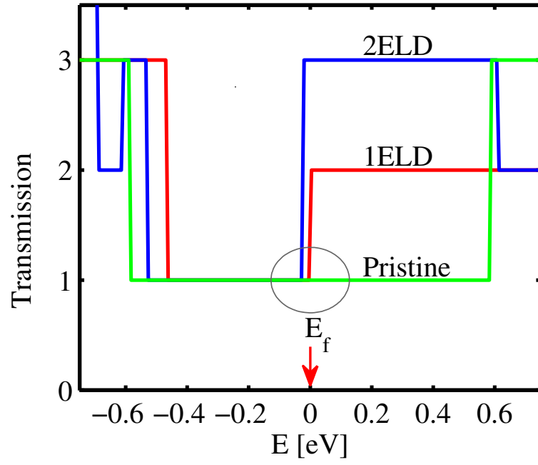
FIG. 2: The transmission function for three different structures: i) The pristine ZGNR(20), ii) ELD-ZGNR(10,10), and iii) 2ELD-ZGNR(8,4,8).
