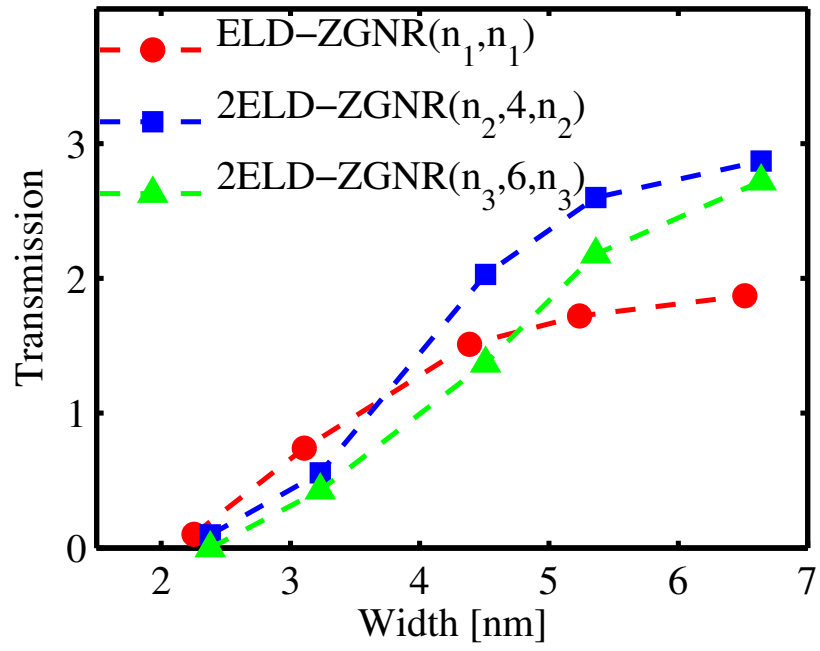
FIG. 6: Transmission at E = 0.2 eV for three different structures as indicated versus their width. The length is assumed to be constant at 250 nm.
