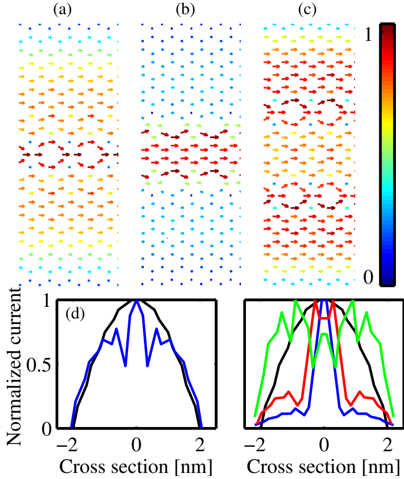
FIG. 3: Normalized current spectrum at E = 0.2 eV for (a) ELD-ZGNR(10,10), (b) 2ELD-ZGNR(8,4,8), and (c) 2ELD(7,6,7). (d) The current in the cross section of ZGNR(20) (black line) and ELD-ZGNR(10,10) (blue line). (e) The current in the cross section of ZGNR(20) (black line), 2ELD-ZGNR(9,2,9) (blue line), 2ELD-ZGNR(8,4,8) (red line), and 2ELD-ZGNR(7,6,7) (green line).
