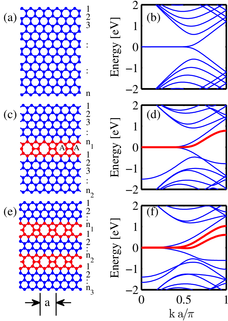
FIG. 1: The geometrical structure of (a) ZGNR( n ), (c) ELD-ZGNR( n_1, n_2 ), and (e) 2ELD-ZGNR( n_1, n_2, n_3 ). The bandstructure of (b) ZGNR(20), (d) ELD-ZGNR(10,10), and (f) 2ELD-ZGNR(8,4,8). The bandstructure of ZGNR(20) is folded for a better comparison. The translation vector length is a = 0.49 nm. The n , n_1 , n_2 and n_3 indicate the number of zigzag edges on the top, bottom, and middle of the ELD regions as indicated.
