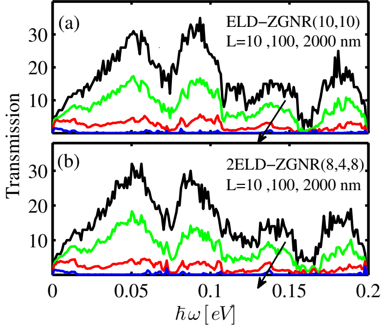
FIG. 7: Phonon transmission probability of (a) ELD-ZGNR(10,10) and (b) 2ELD-ZGNR(8,4,8). Rough edges are assumed and the length L of the channel is varied. The arrows indicate increasing values of channel length L , 10 nm-green, 100 nm-red, 2000 nm-blue lines. Black lines: The phonon transmission of the channels with line defects but without roughness.
