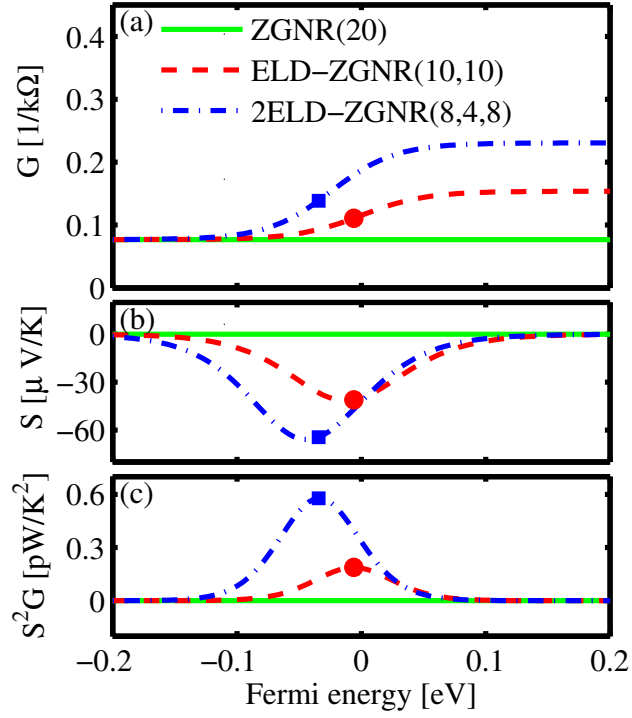
FIG. 9: (a) Electrical conductance, (b) Seebeck coefficient, and (c) thermoelectric power factor of pristine ZGNR(20), ELD-ZGNR(10,10), and 2ELD-ZGNR(8,4,8) channels with perfect edges. The dots indicate the Fermi energy values at which the peak of the power factor occurs for the ELD and 2ELD channels.
