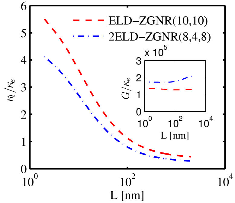
FIG. 8: The ratio of the phononic to the electronic thermal conductivity versus channel length L for the ELD and 2ELD structures as noted. Inset: The ratio of the electronic conductivity to the electronic part of the thermal conductivity versus channel length L .
